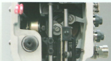
Sewing kinematics with increased needle bar stroke enables the processing of highly-flexible threads in size 80/3-15/3 syn.
